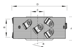
SmartJointer airFace
